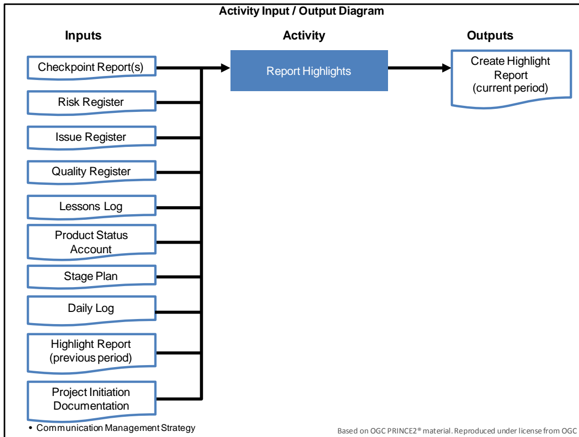
Fig 16.6 Report Highlights
