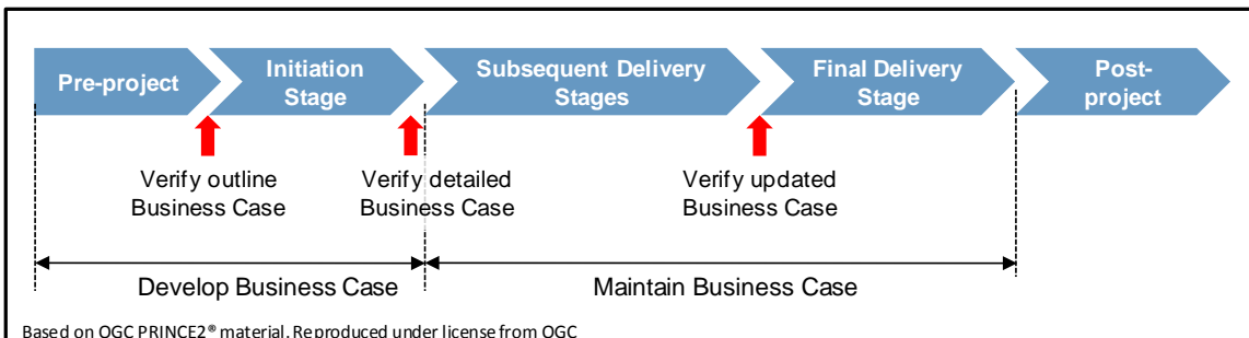
Fig 5.3 Verification Points
