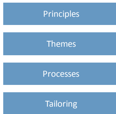
Fig 1.2 PRINCE2 Structure
